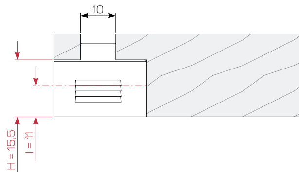
STANDARD CON CODOLO STANDARD WITH DOWEL
